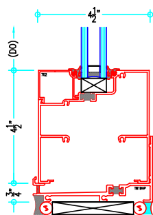
TALL SILL OPTION #1
