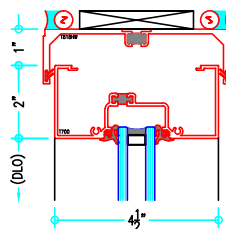
COMP CHANNEL OPTION #2
